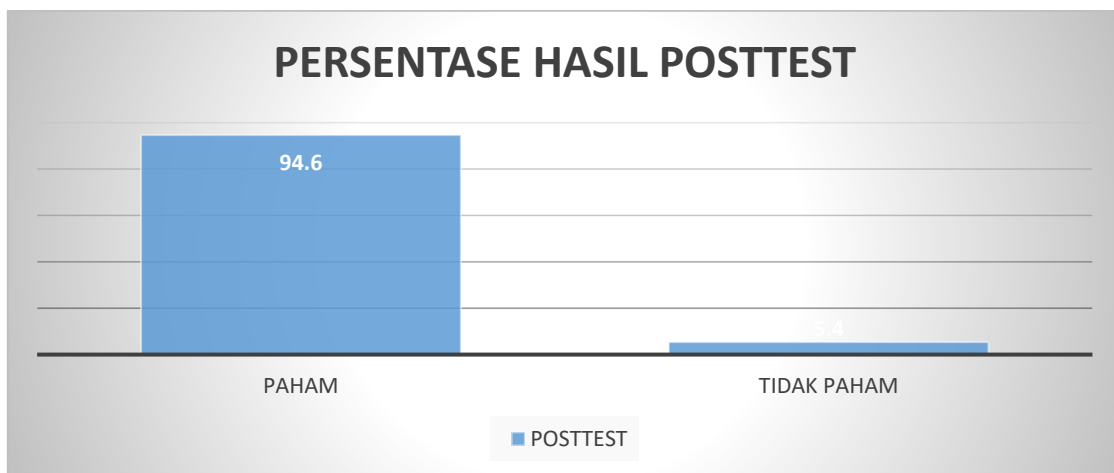
Gambar 2. Diagram Batang Persentase Hasil Posttest
