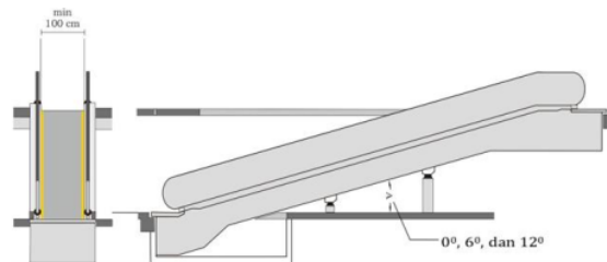
Gambar 2. 1 Detail Lantai Berjalan
