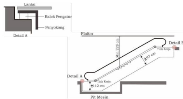
Gambar 19. Detail Eskalator
